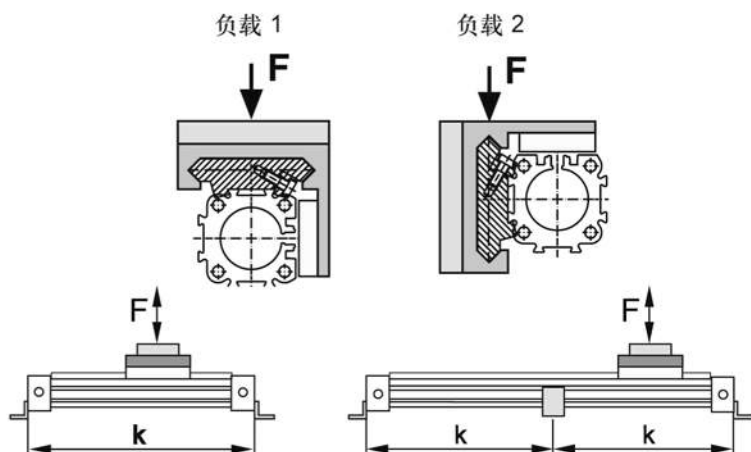
允许无支撑长度MB-SL25, MB-SL32
