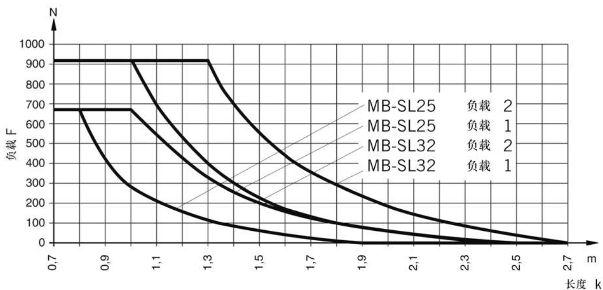
允许无支撑长度MB-SL25, MB-SL32
